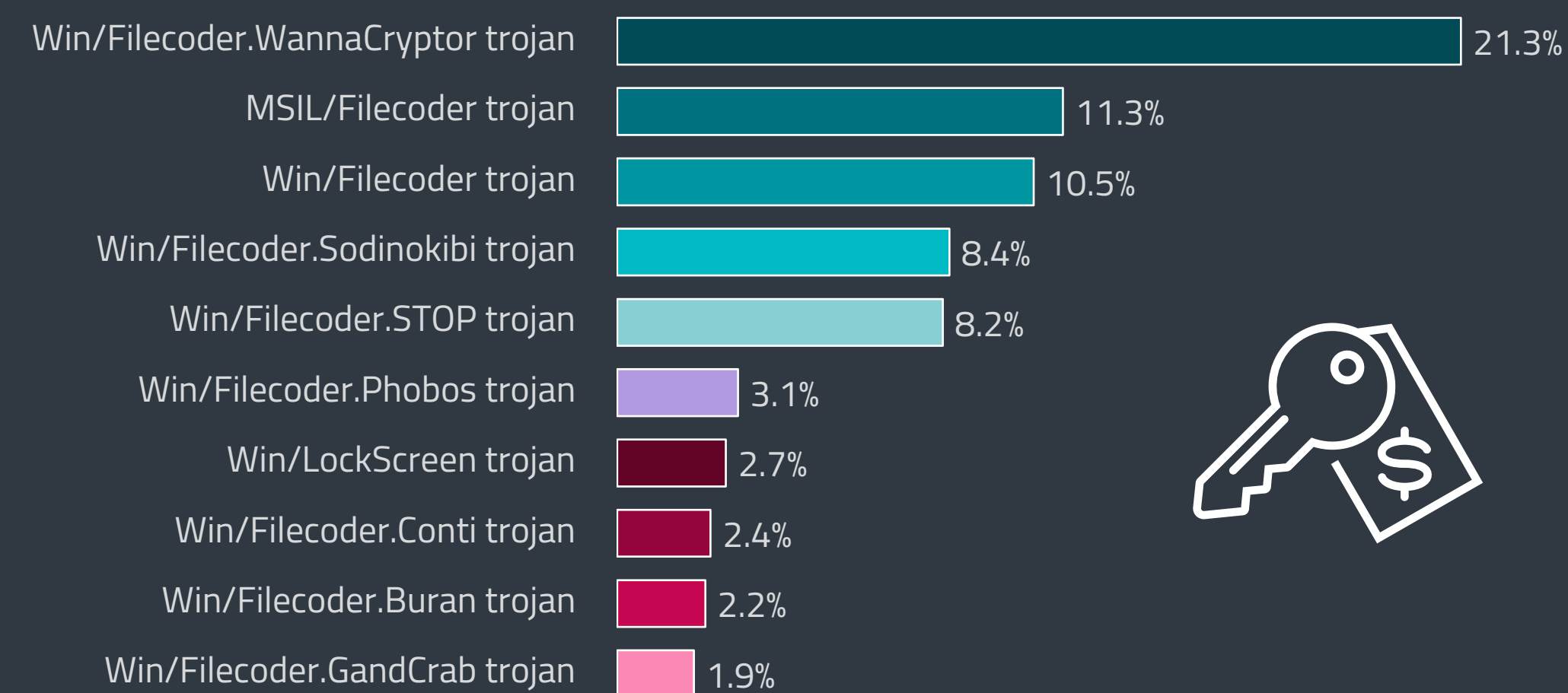
Top 10 ransomware families in T2 2021 (% of ransomware detections)
