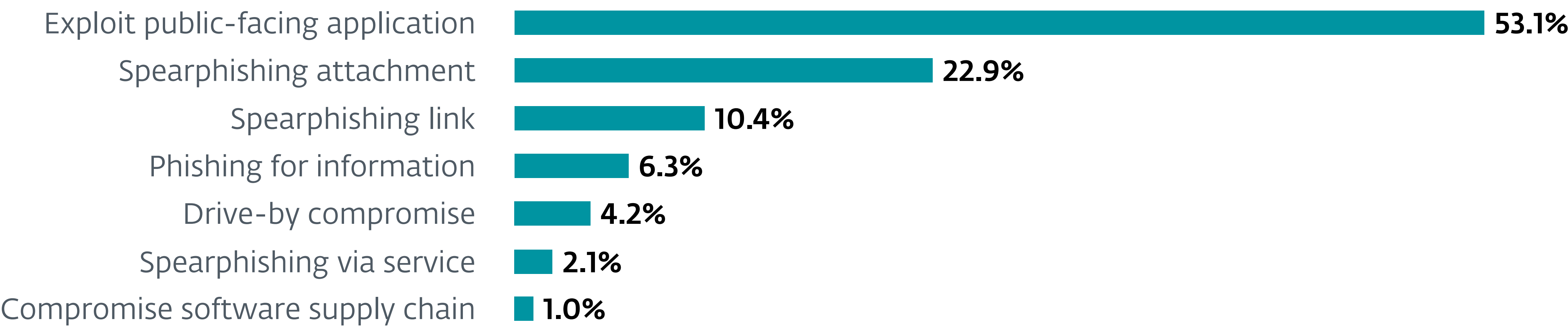
Initial access techniques used by Russia-aligned APT groups
