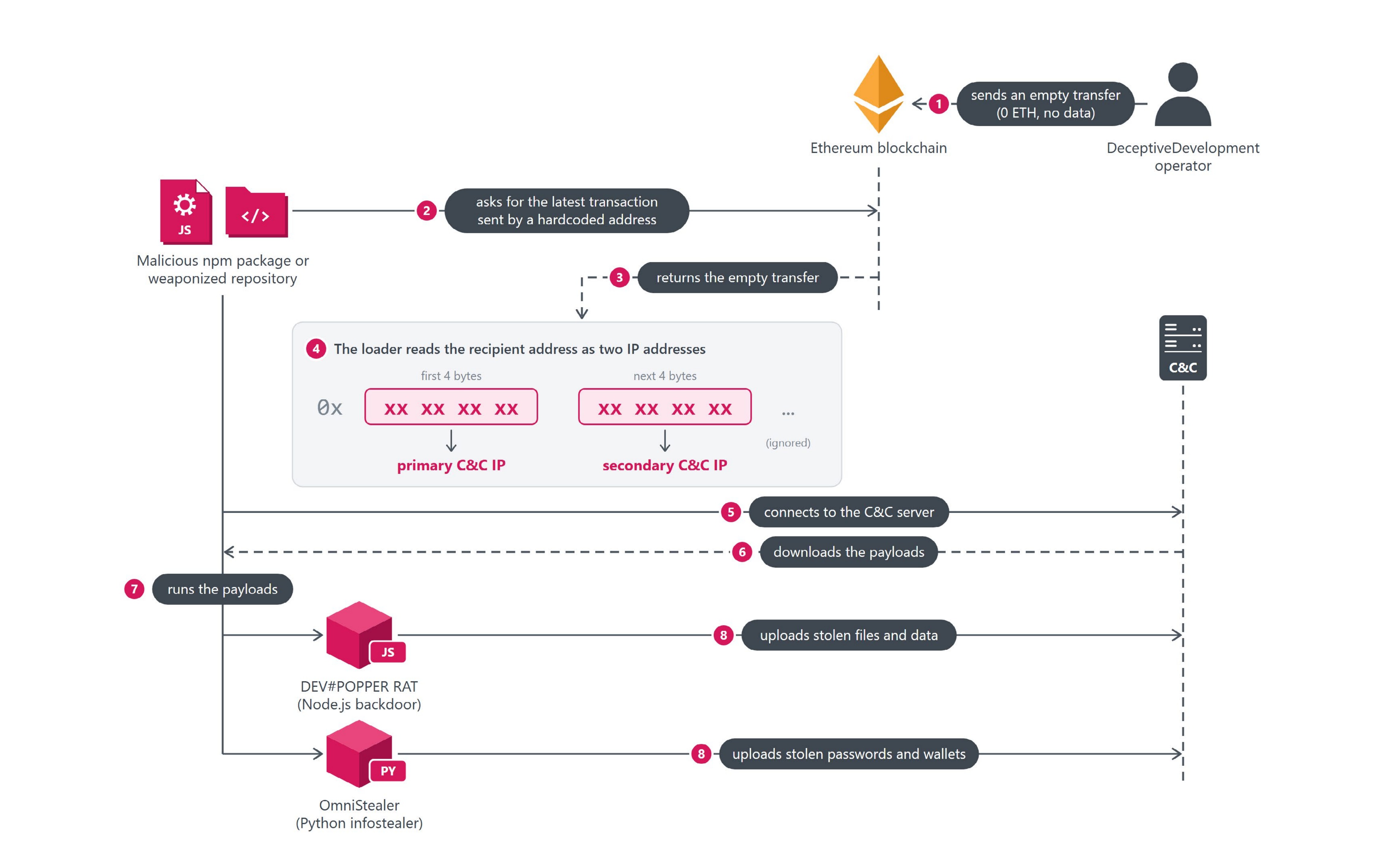
Figure 5. Execution chain using NullReceiver
