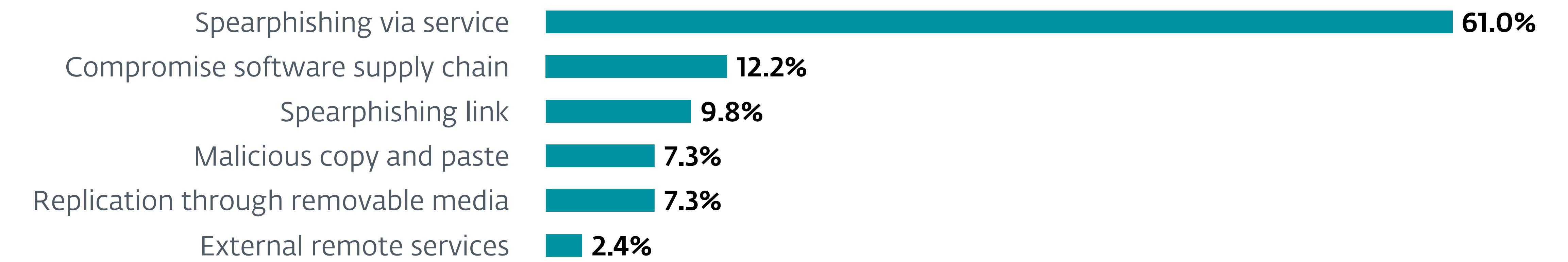
Initial access techniques used by North Korea-aligned APT groups
