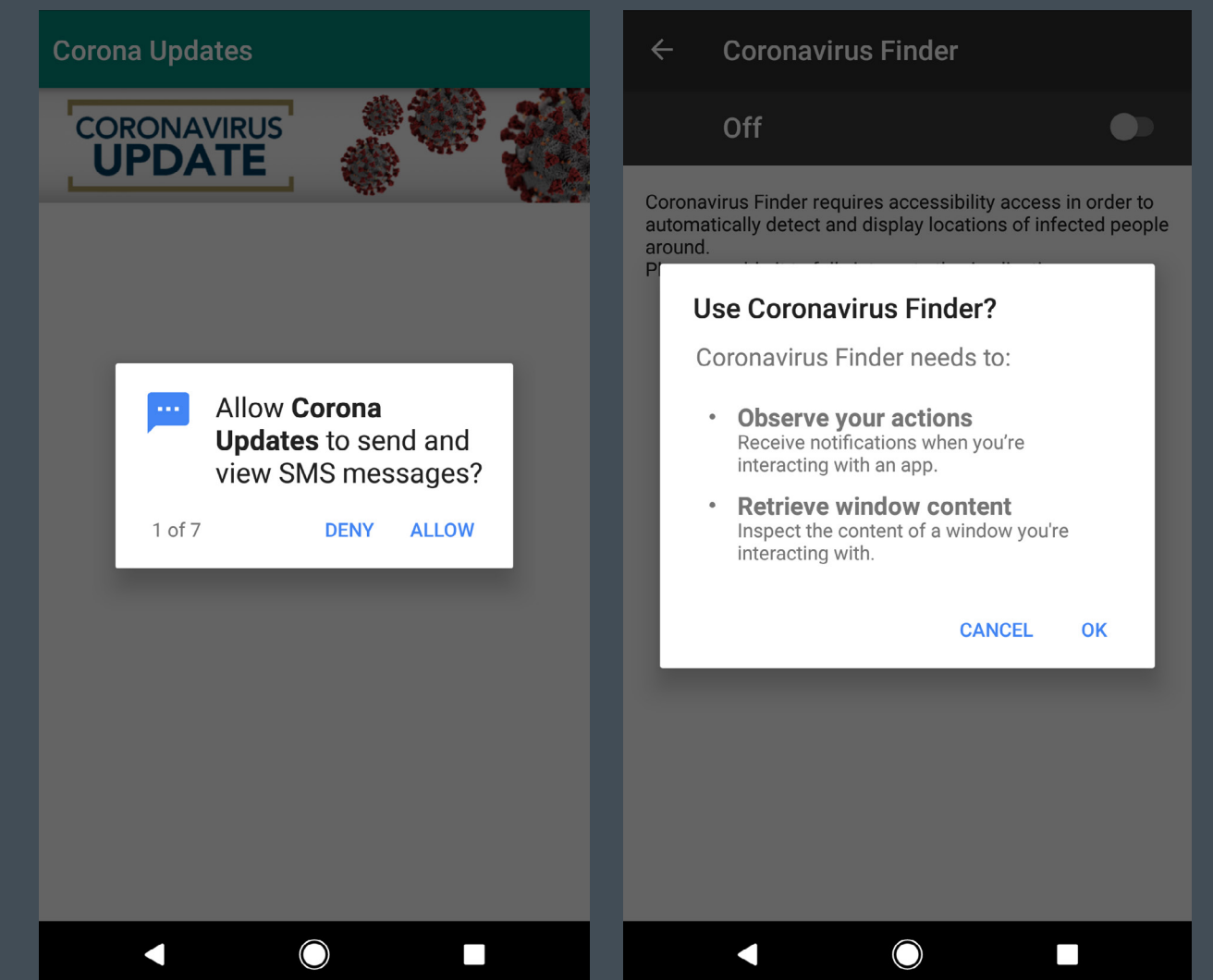
Examples of coronavirus-themed Android malware permission requests
