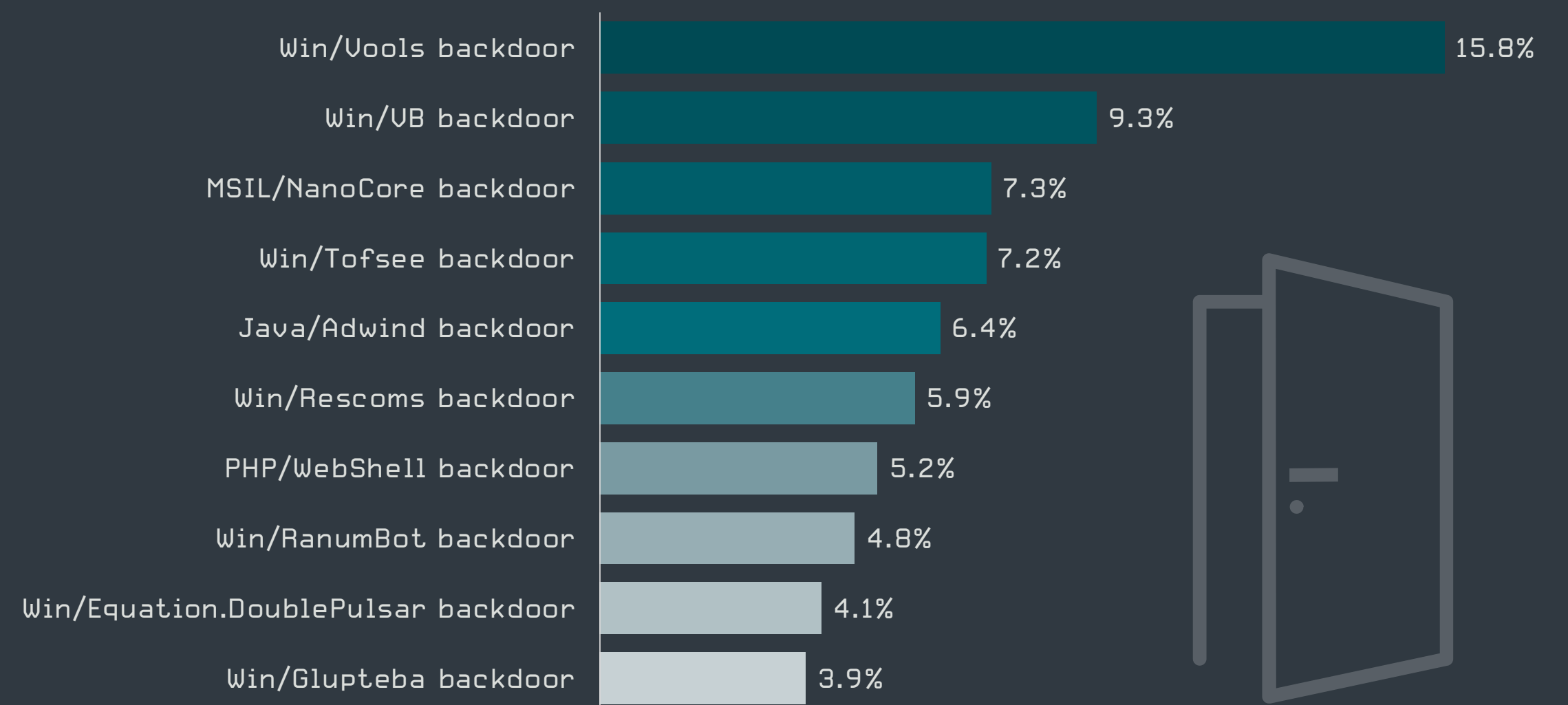
Top 10 backdoor families in Q1 2020 [% of backdoor detections]
