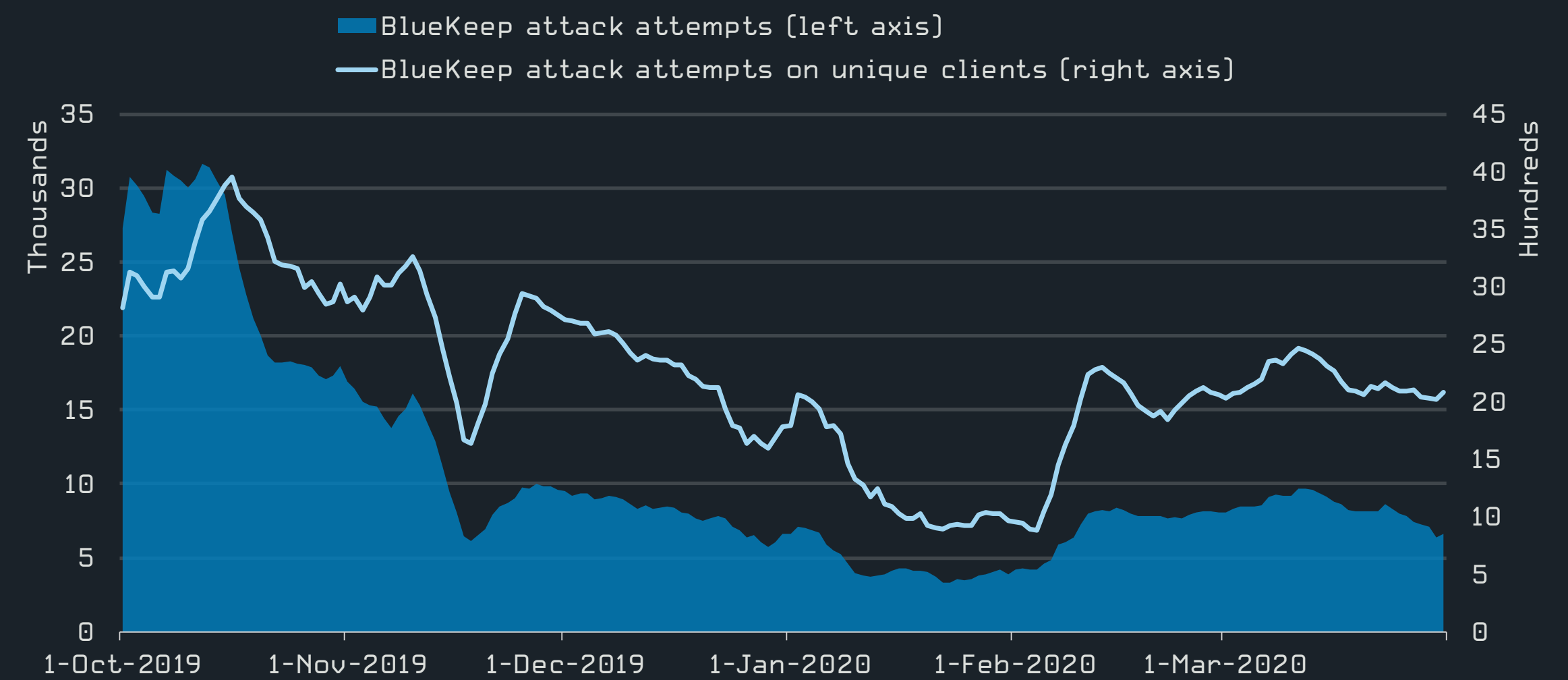
Trends of BlueKeep attack attempts in Q4 2019-Q1 2020, seven-day moving average
