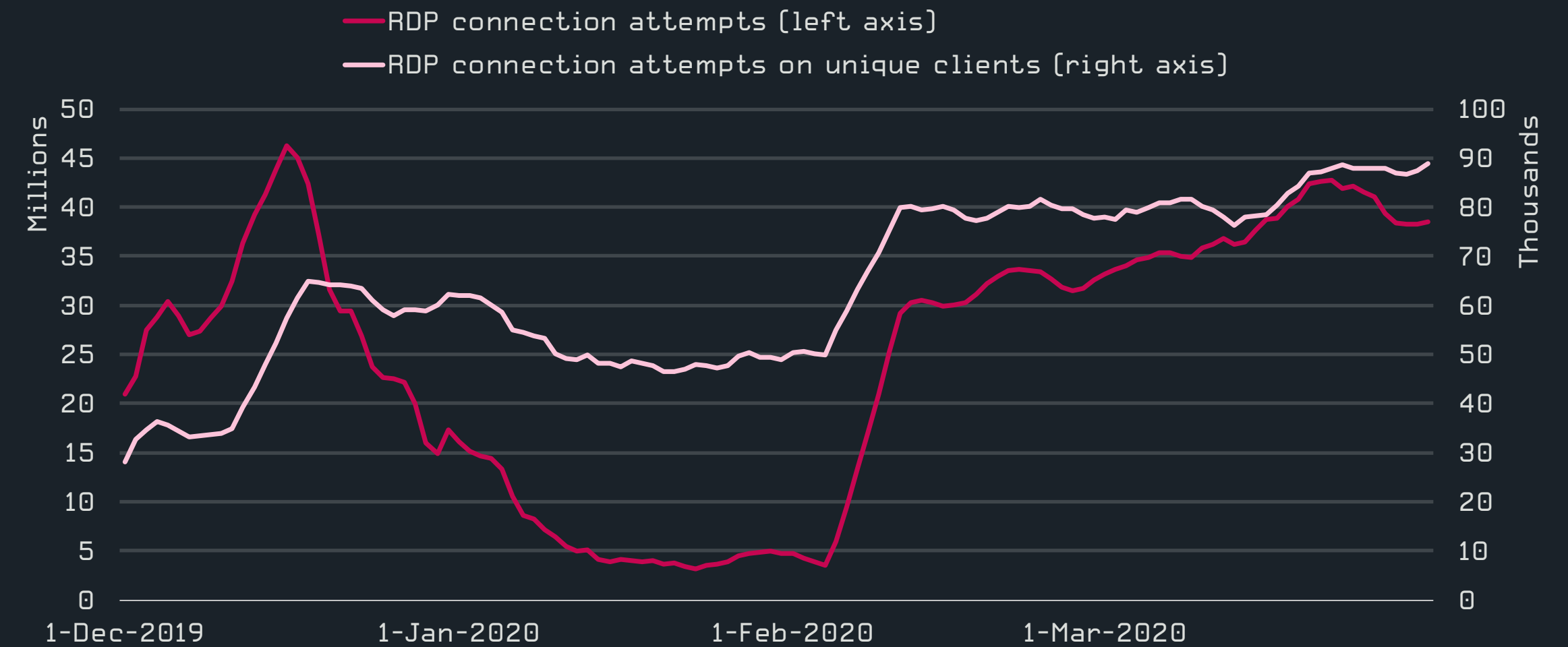
Trends of RDP connection attempts in Q4 2019-Q1 2020, seven-day moving average 2
